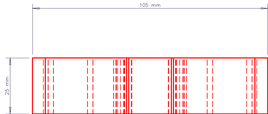
SIDE VIEW (1 : 1)
